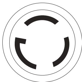
Figure 15 - 120 VAC, 30 Amp Receptacle
