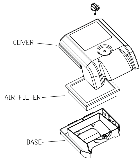
Figure 24 - 10kW Air Filter (Part Number 073111)
