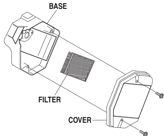
Figure 24 - 10kW Air Filter (Part Number 073111)
