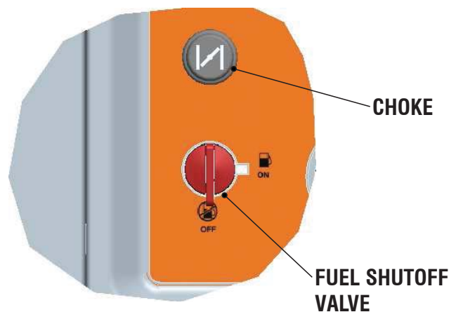
Figure 19 - Fuel Shut-off Valve
