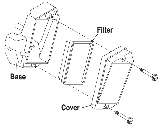
Figure 22 - 3.6kW Air Filter (Part Number 078601)
