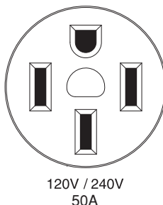
Figure 13 - Prise de 120/240 Volts CA, 50 Amp
