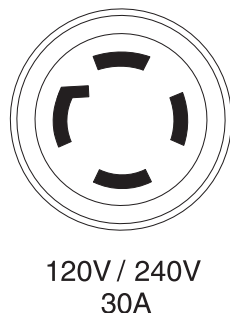
Figure 12 - Prise de 120/240 Volts CA, 30 Amp
