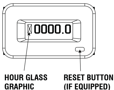
Figure 10 – Hourmeter
