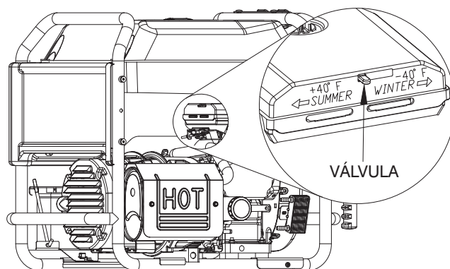
Figure 8 - Generator Controls
