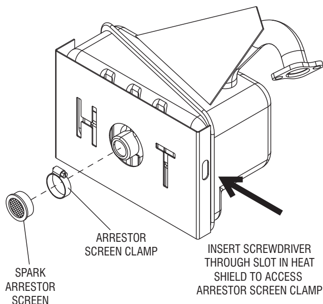
Figure 25 - 3.6kW Spark Arrestor
