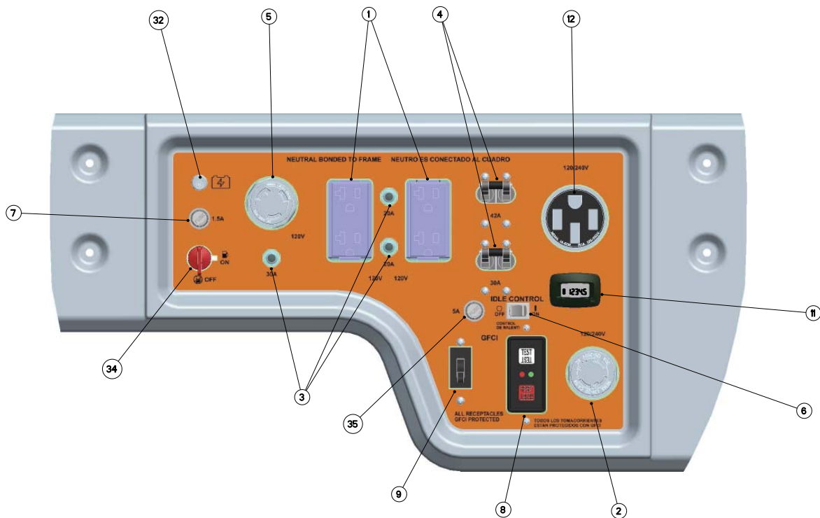
Figure 7 - 10,000 Watt Control Panel
