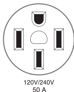
Figure 13 - 120/240 VAC, 50 Amp Receptacle
