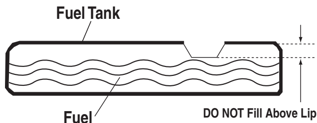
Figure 17 - Fuel Tank
